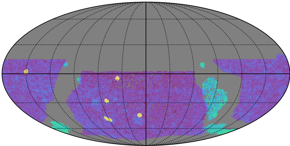
too_elab_r32_d2_gz_v3.4_10yrs WFD g band: NVisits
