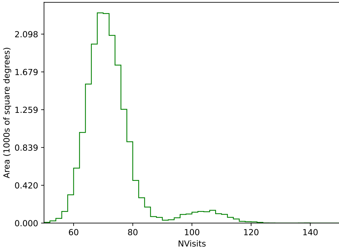
too_elab_r32_d2_gz_v3.4_10yrs WFD g band: NVisits
