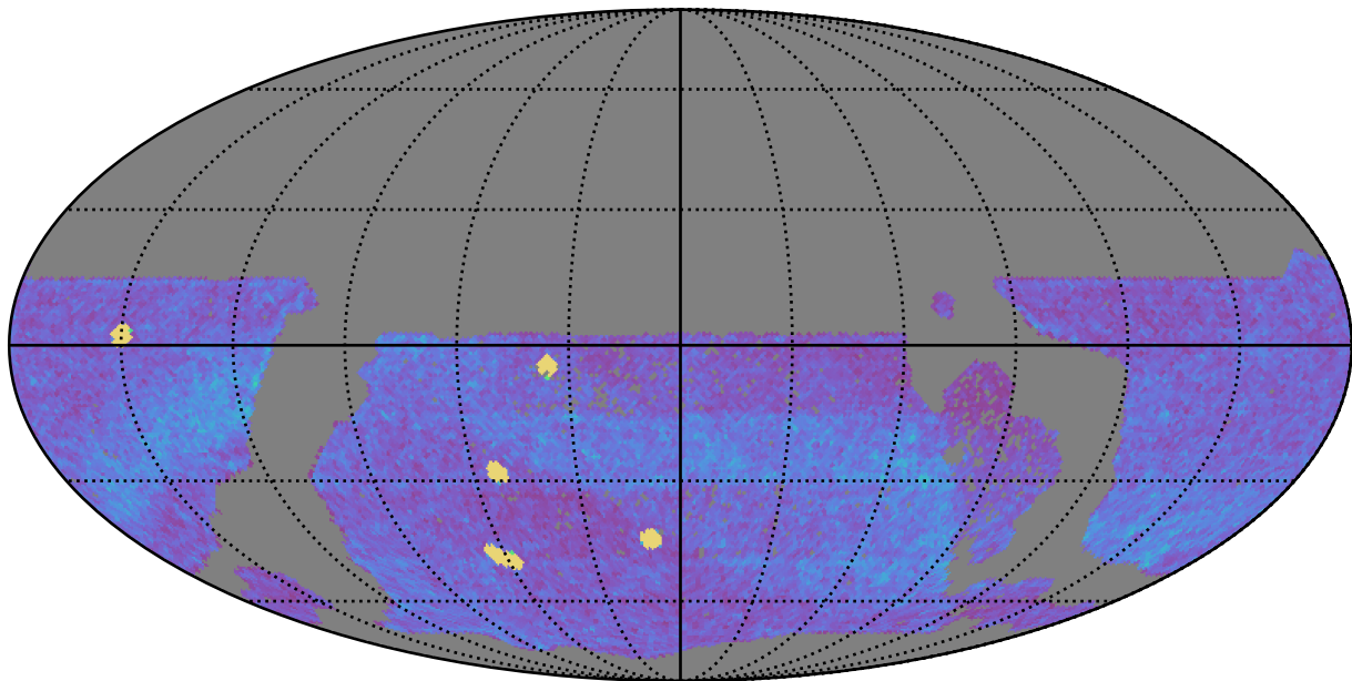
too_elab_r32_d2_gz_v3.4_10yrs WFD all bands: NVisits
