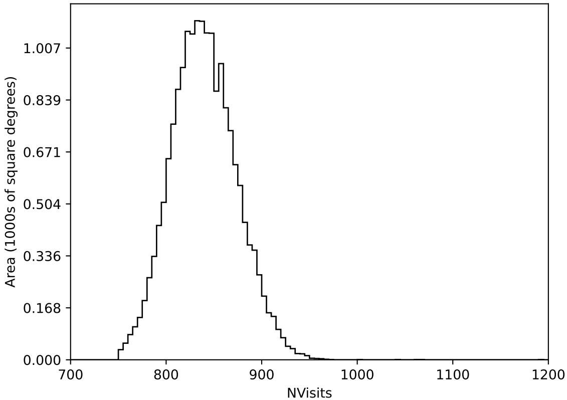
too_elab_r32_d2_gz_v3.4_10yrs WFD all bands: NVisits
