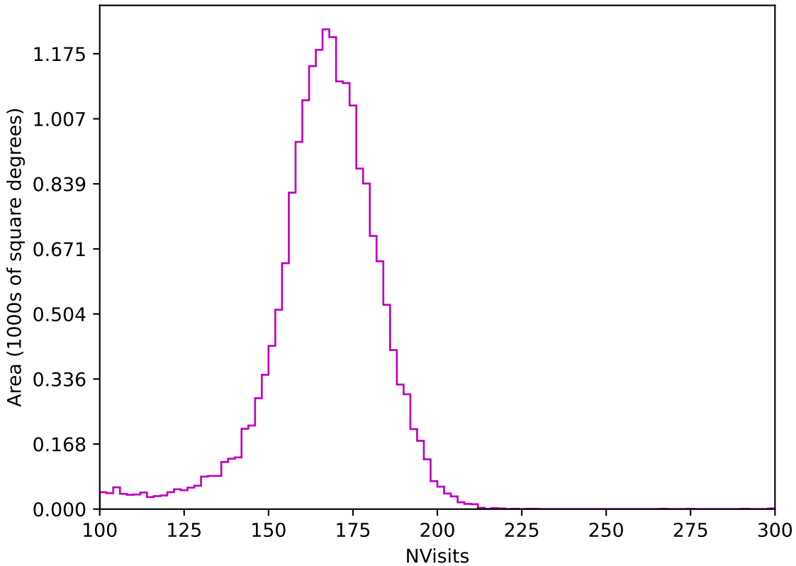
too_elab_r32_d2_gz_v3.4_10yrs All sky z band: NVisits
