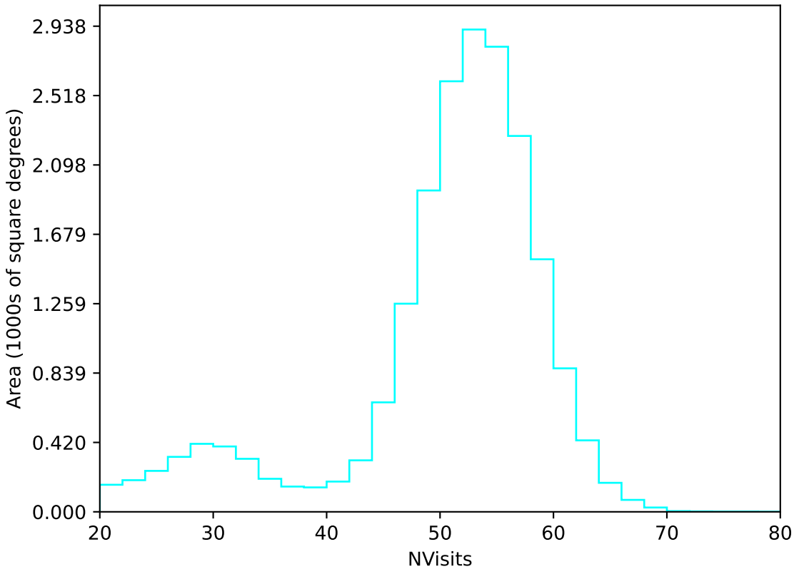
too_elab_r32_d2_gz_v3.4_10yrs All sky u band: NVisits
