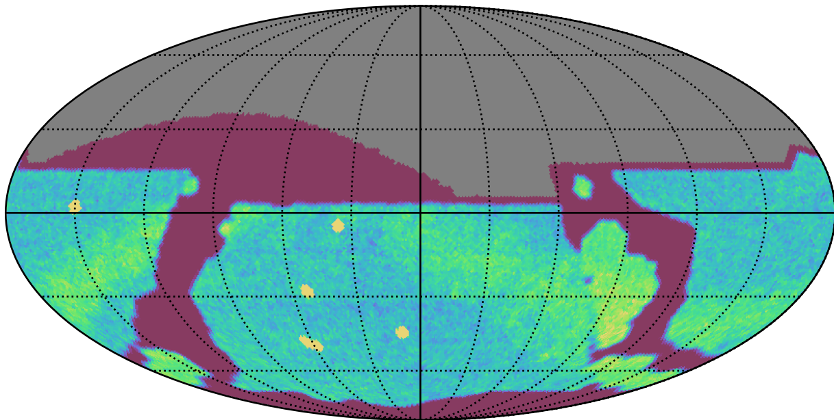
too_elab_r32_d2_gz_v3.4_10yrs All sky r band: NVisits
