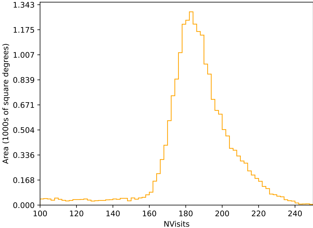
too_elab_r32_d2_gz_v3.4_10yrs All sky r band: NVisits
