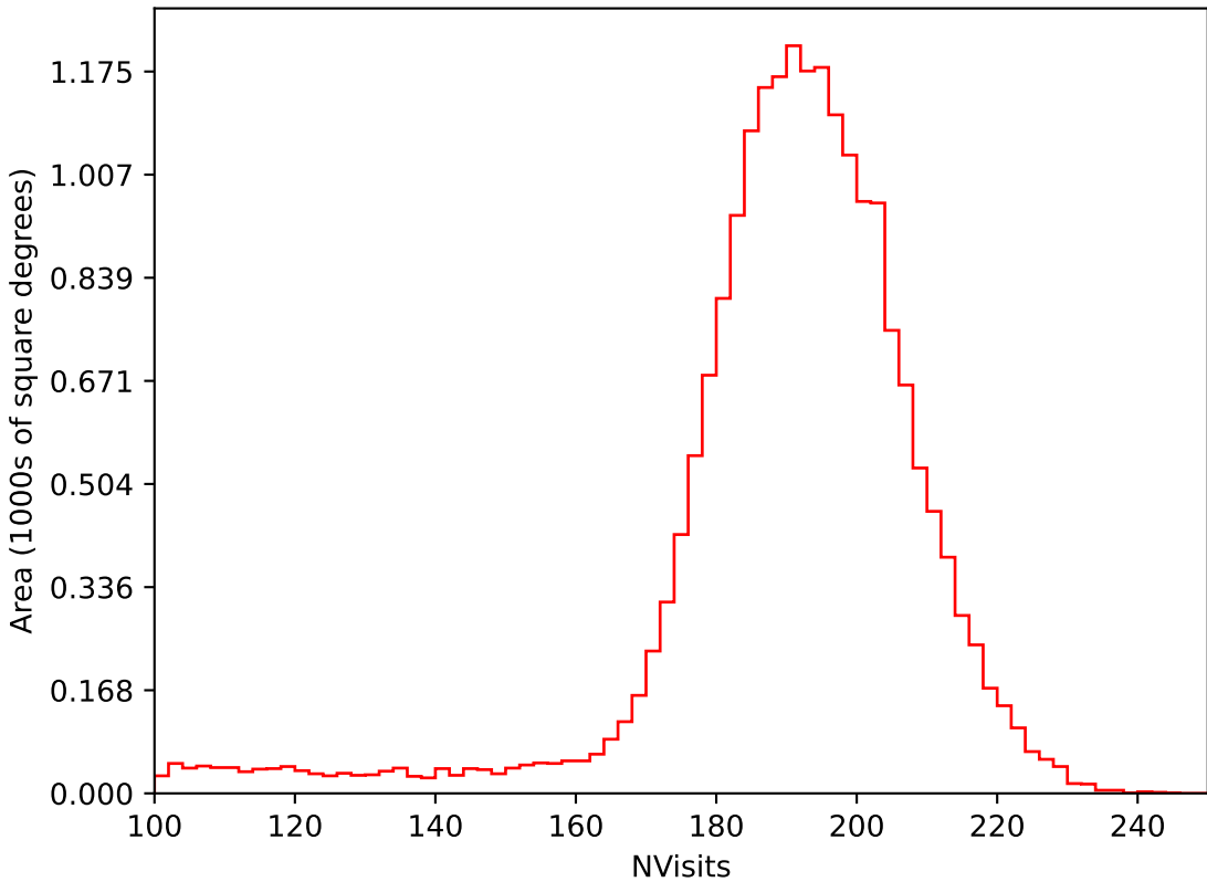
too_elab_r32_d2_gz_v3.4_10yrs All sky i band: NVisits
