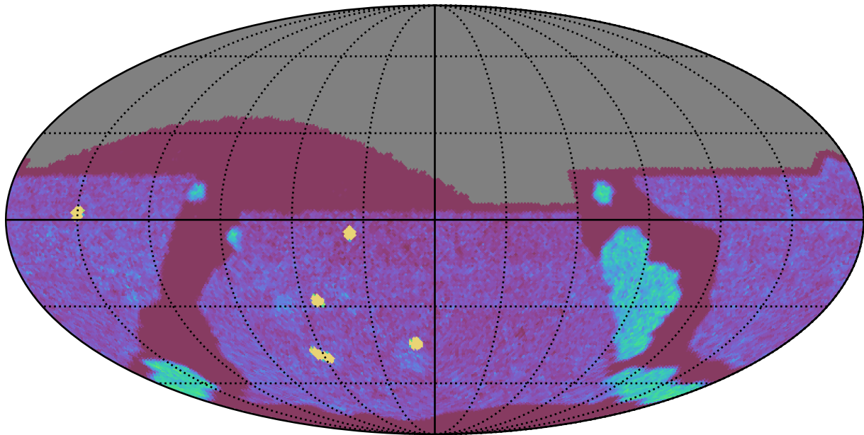
too_elab_r32_d2_gz_v3.4_10yrs All sky g band: NVisits
