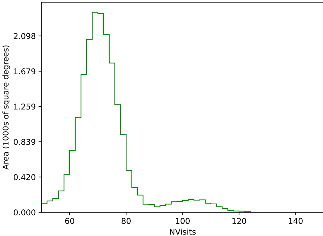
too_elab_r32_d2_gz_v3.4_10yrs All sky g band: NVisits
