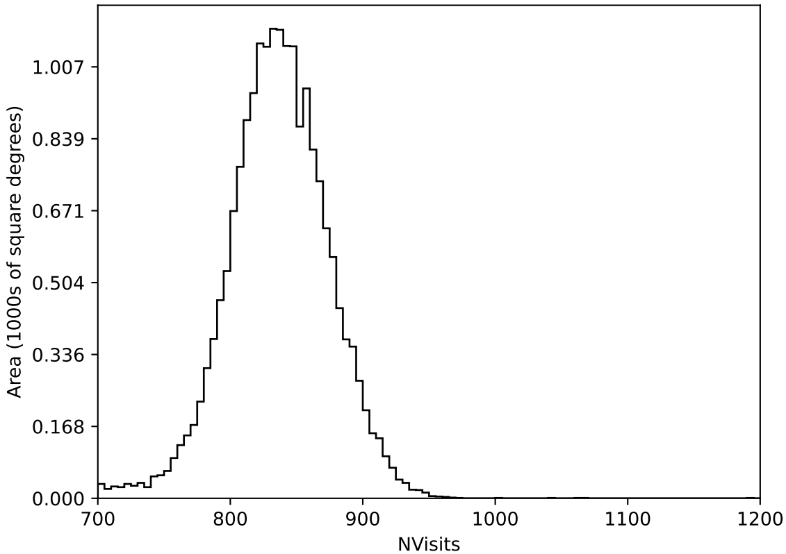
too_elab_r32_d2_gz_v3.4_10yrs All sky all bands: NVisits
