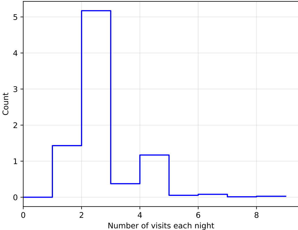
too_elab_r32_d2_gz_v3.4_10yrs WFD: NVisitsPerNight
