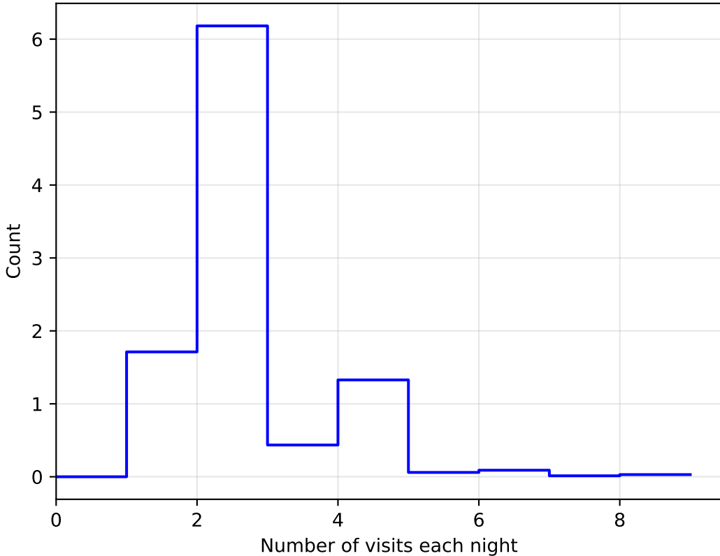
too_elab_r32_d2_gz_v3.4_10yrs All sky: NVisitsPerNight
