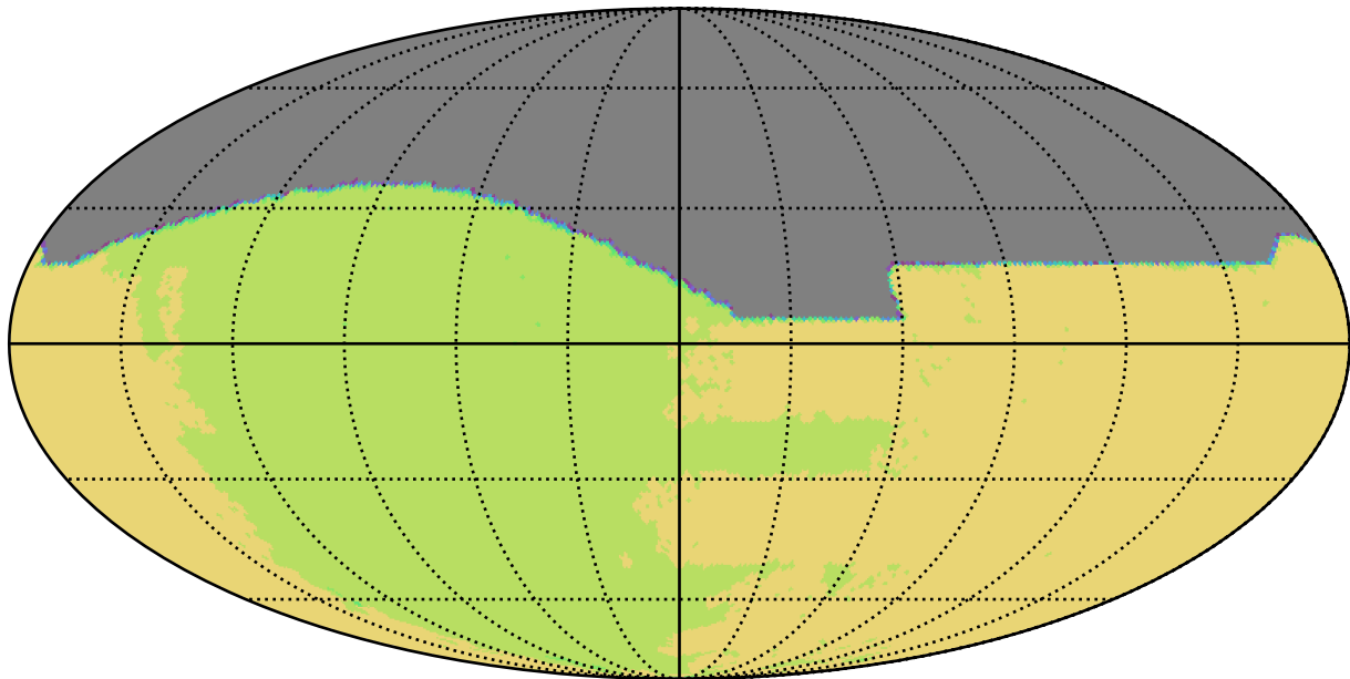
too_elab_r32_d2_gz_v3.4_10yrs All sky all bands: NSeasons
