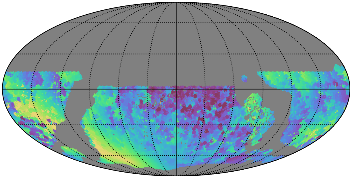
too_elab_r32_d2_gz_v3.4_10yrs WFD y band: Min solarElong
