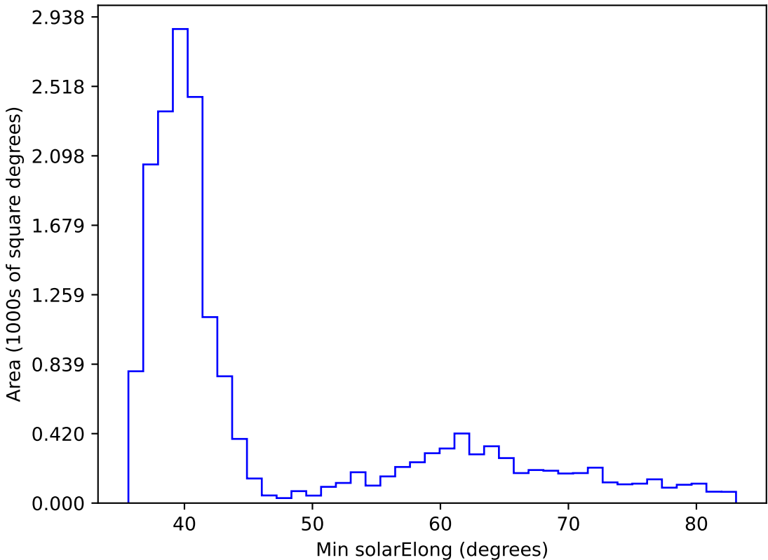
too_elab_r32_d2_gz_v3.4_10yrs WFD all bands: Min solarElong
