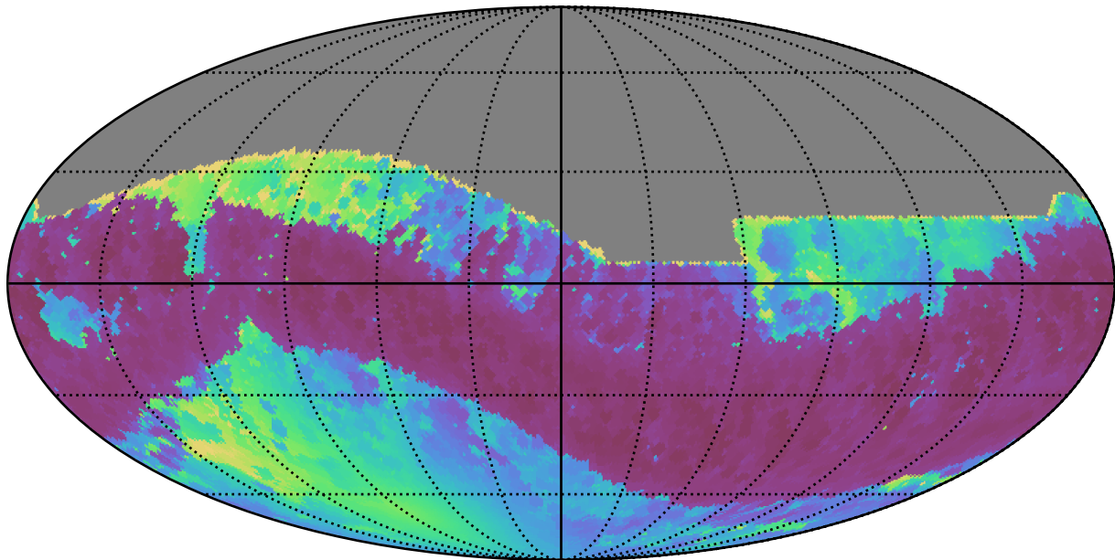
too_elab_r32_d2_gz_v3.4_10yrs All sky z band: Min solarElong
