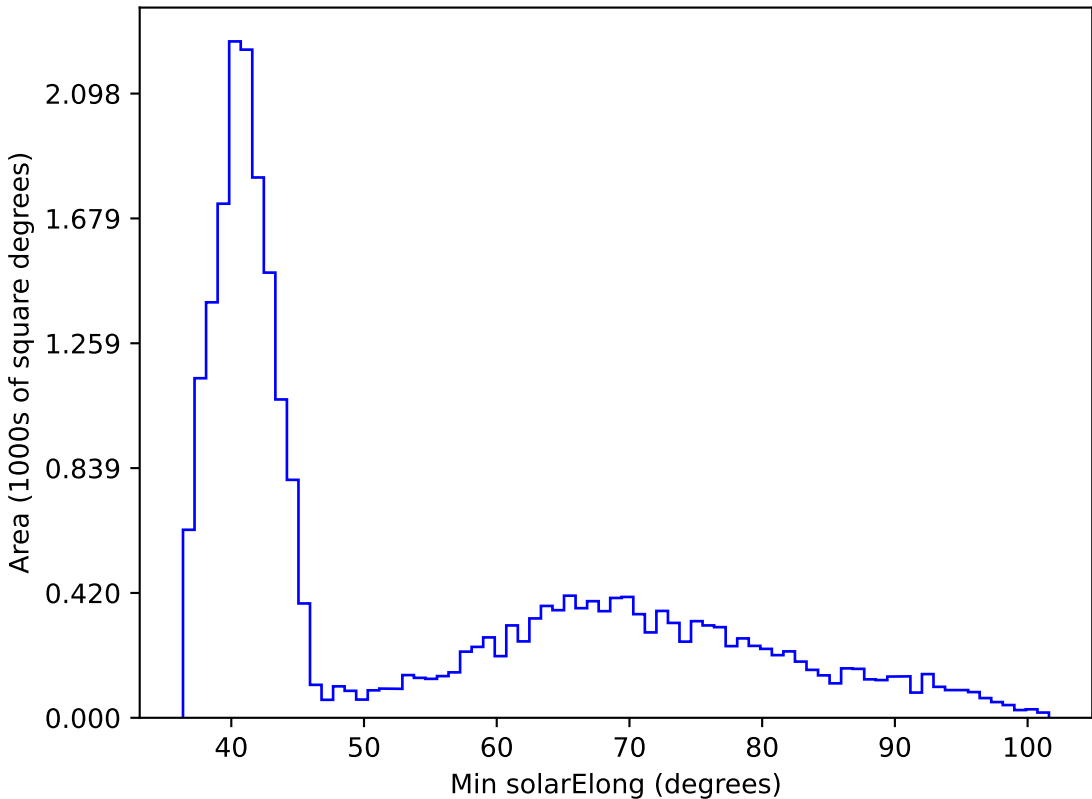
too_elab_r32_d2_gz_v3.4_10yrs All sky z band: Min solarElong
