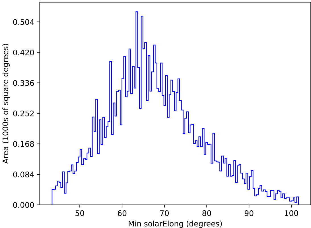
too_elab_r32_d2_gz_v3.4_10yrs All sky y band: Min solarElong
