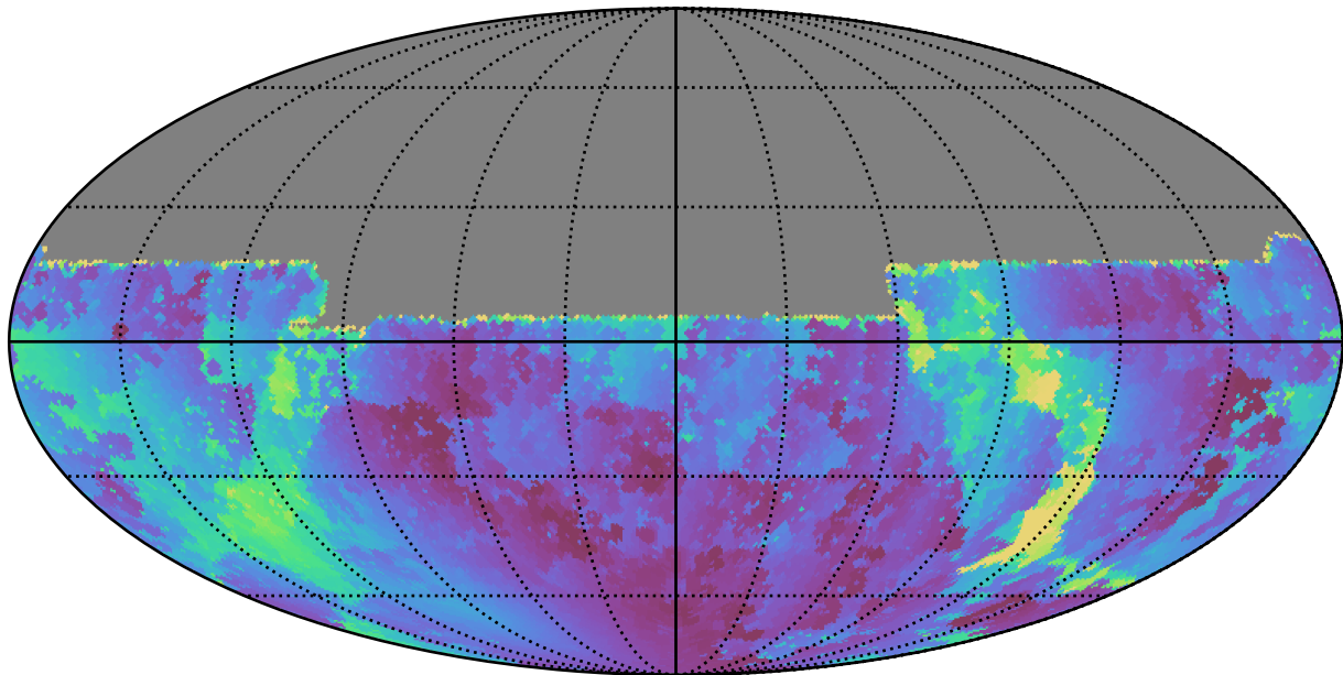
too_elab_r32_d2_gz_v3.4_10yrs All sky u band: Min solarElong
