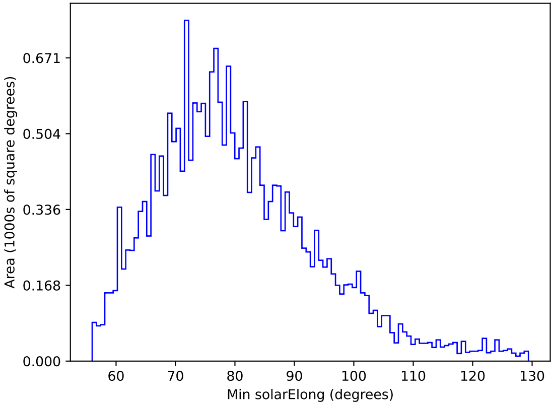
too_elab_r32_d2_gz_v3.4_10yrs All sky u band: Min solarElong
