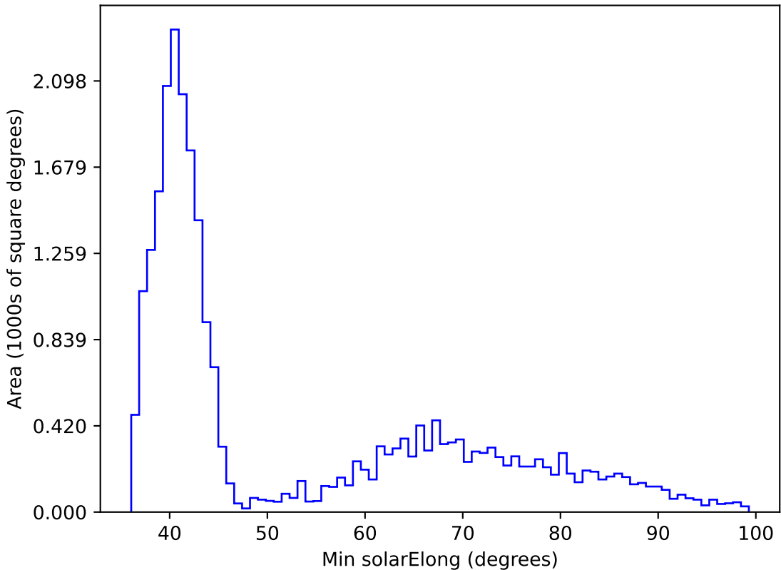
too_elab_r32_d2_gz_v3.4_10yrs All sky i band: Min solarElong
