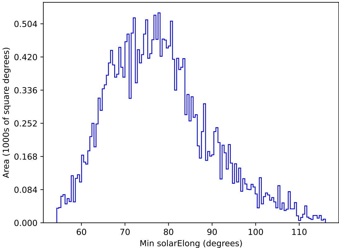
too_elab_r32_d2_gz_v3.4_10yrs All sky g band: Min solarElong
