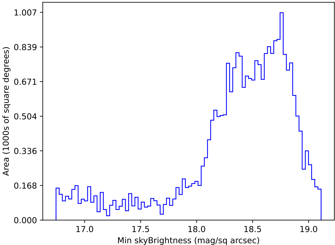
too_elab_r32_d2_gz_v3.4_10yrs Yr 1 z band: Min skyBrightness
