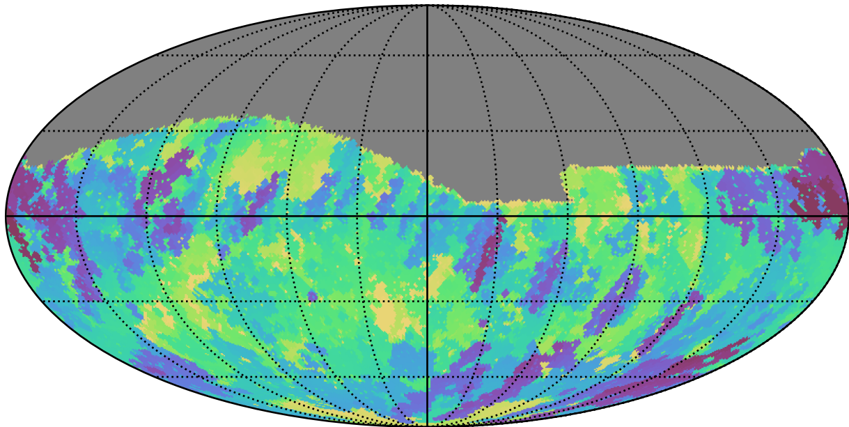
too_elab_r32_d2_gz_v3.4_10yrs Yr 1 r band: Min skyBrightness
