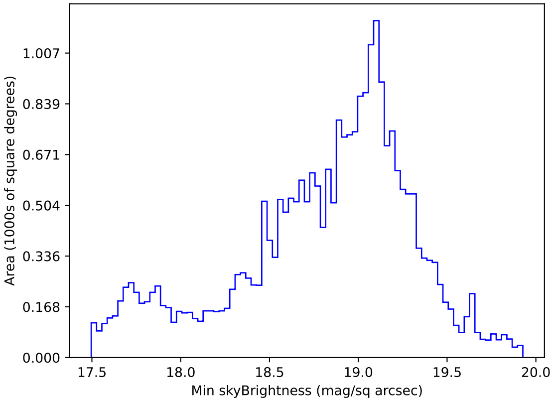
too_elab_r32_d2_gz_v3.4_10yrs Yr 1 i band: Min skyBrightness
