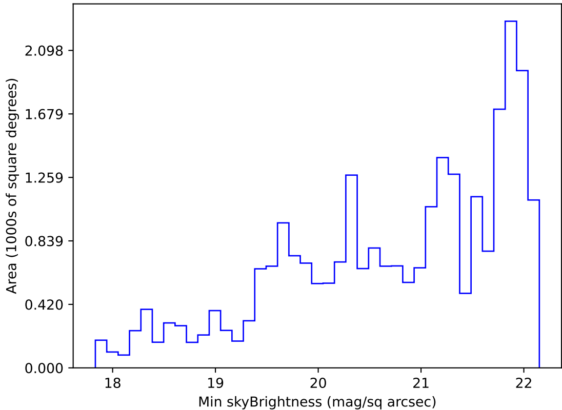
too_elab_r32_d2_gz_v3.4_10yrs Yr 1 g band: Min skyBrightness
