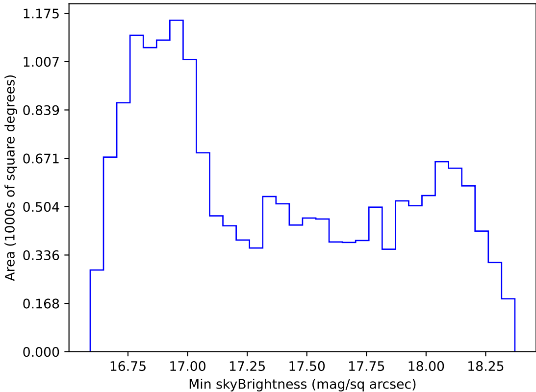
too_elab_r32_d2_gz_v3.4_10yrs WFD z band: Min skyBrightness
