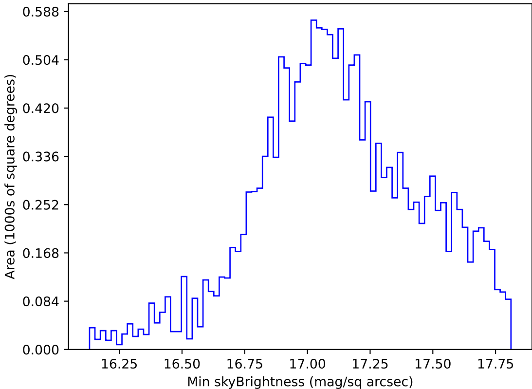
too_elab_r32_d2_gz_v3.4_10yrs WFD y band: Min skyBrightness
