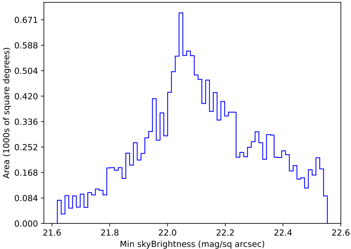
too_elab_r32_d2_gz_v3.4_10yrs WFD u band: Min skyBrightness
