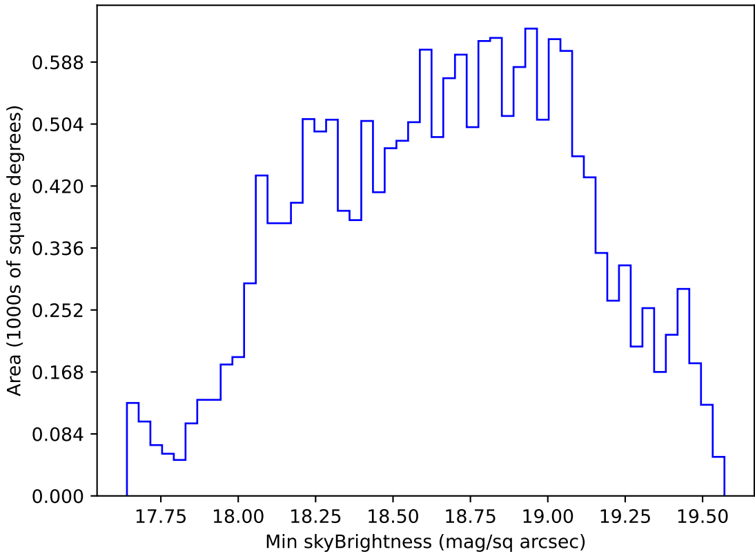
too_elab_r32_d2_gz_v3.4_10yrs WFD r band: Min skyBrightness
