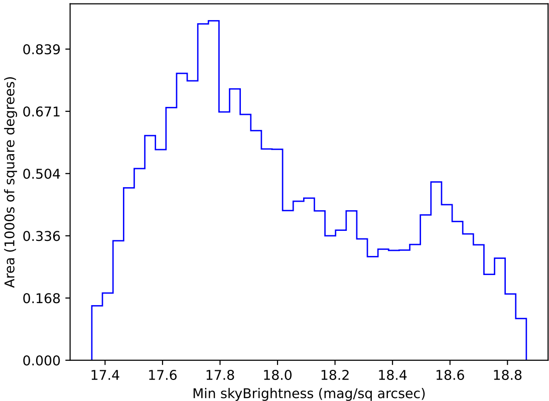
too_elab_r32_d2_gz_v3.4_10yrs WFD i band: Min skyBrightness
