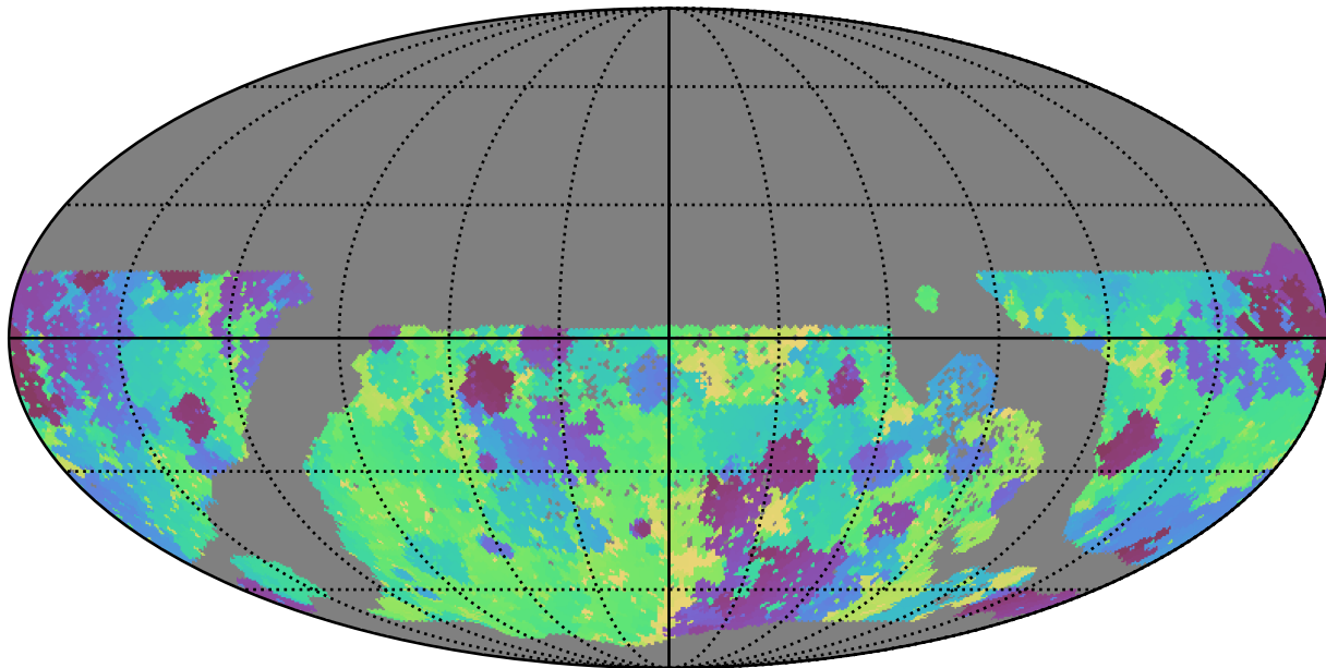
too_elab_r32_d2_gz_v3.4_10yrs WFD g band: Min skyBrightness
