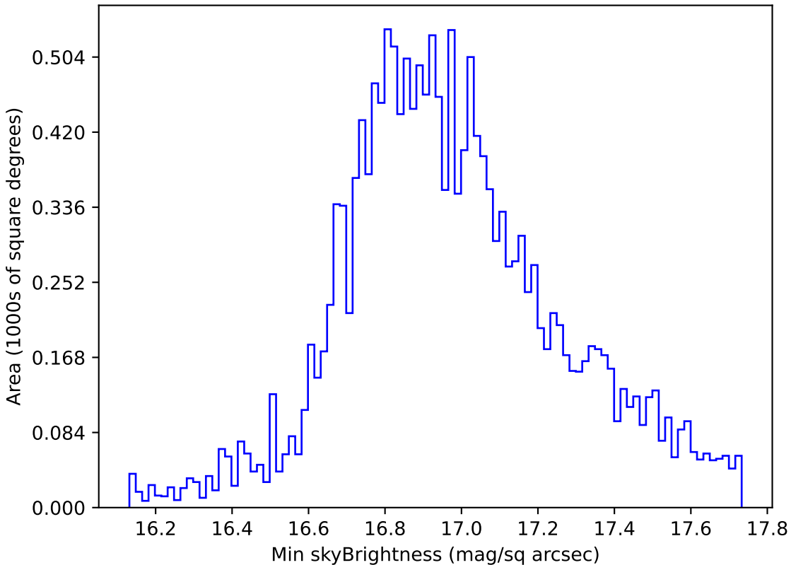
too_elab_r32_d2_gz_v3.4_10yrs WFD all bands: Min skyBrightness
