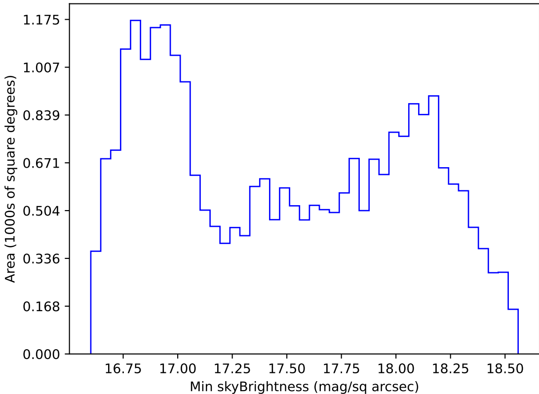
too_elab_r32_d2_gz_v3.4_10yrs All sky z band: Min skyBrightness
