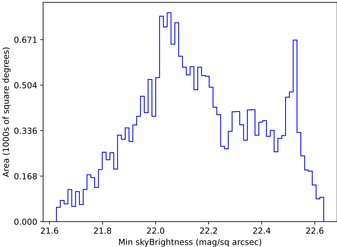
too_elab_r32_d2_gz_v3.4_10yrs All sky u band: Min skyBrightness
