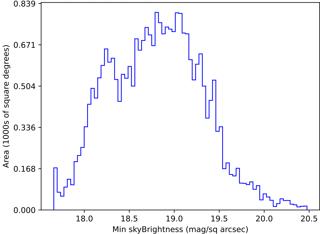
too_elab_r32_d2_gz_v3.4_10yrs All sky r band: Min skyBrightness
