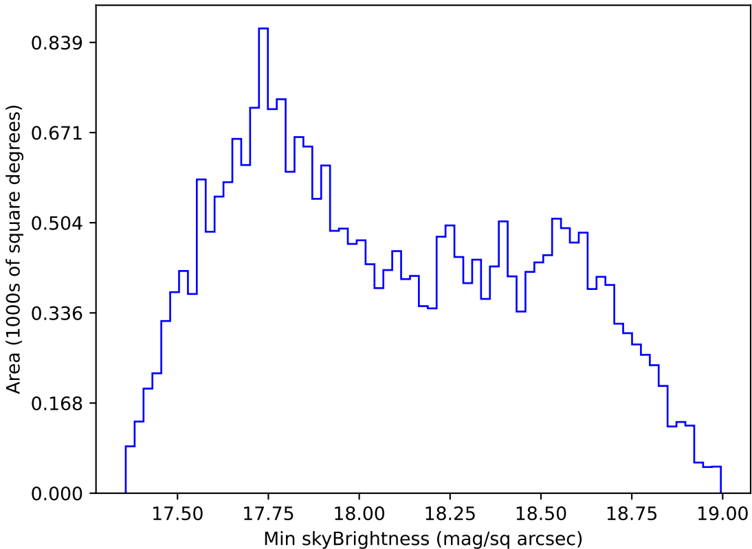
too_elab_r32_d2_gz_v3.4_10yrs All sky i band: Min skyBrightness
