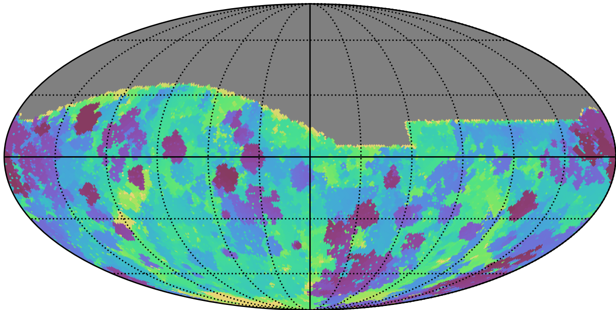
too_elab_r32_d2_gz_v3.4_10yrs All sky g band: Min skyBrightness
