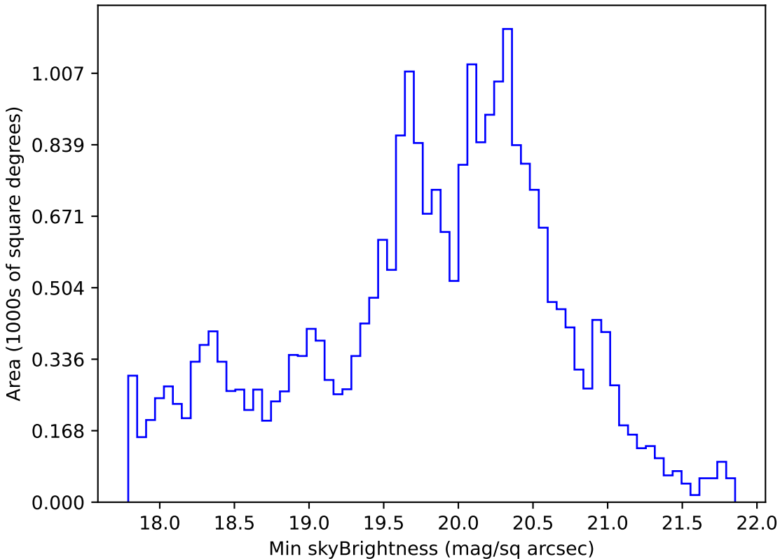
too_elab_r32_d2_gz_v3.4_10yrs All sky g band: Min skyBrightness
