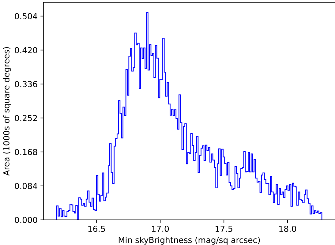
too_elab_r32_d2_gz_v3.4_10yrs All sky all bands: Min skyBrightness
