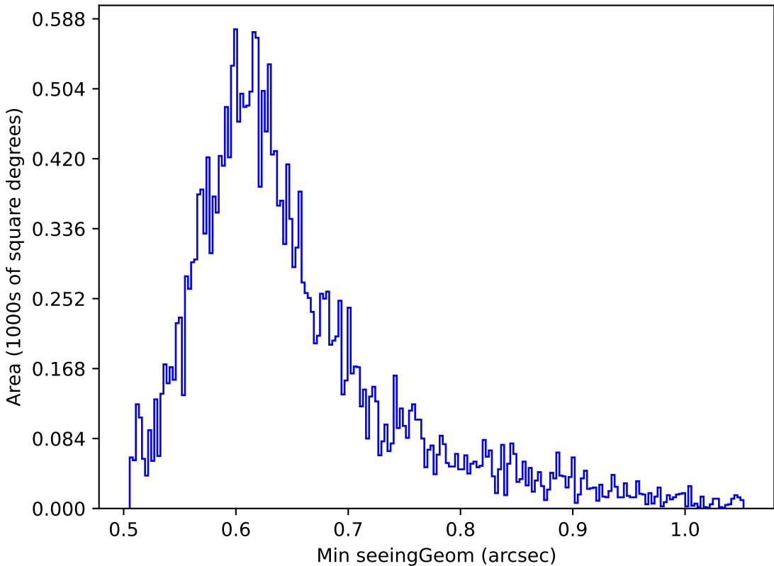
too_elab_r32_d2_gz_v3.4_10yrs Yr 1 z band: Min seeingGeom
