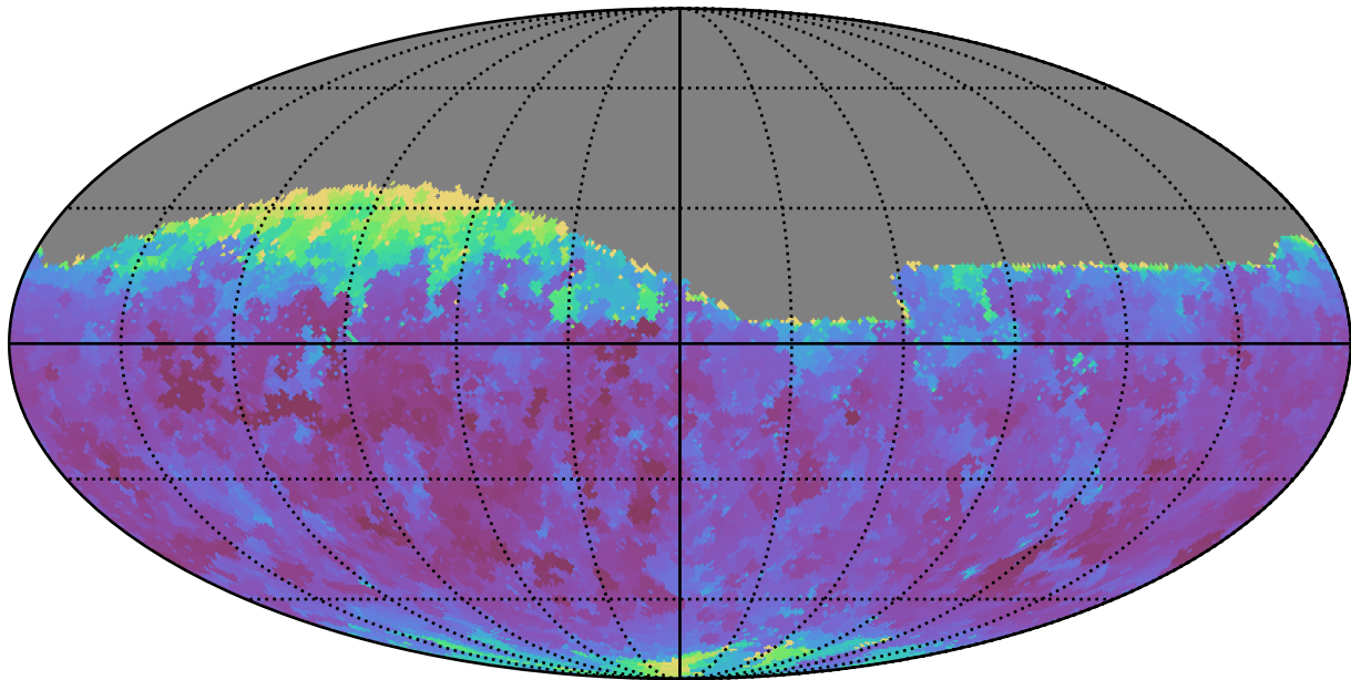
too_elab_r32_d2_gz_v3.4_10yrs Yr 1 r band: Min seeingGeom
