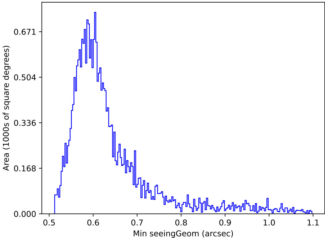
too_elab_r32_d2_gz_v3.4_10yrs Yr 1 i band: Min seeingGeom
