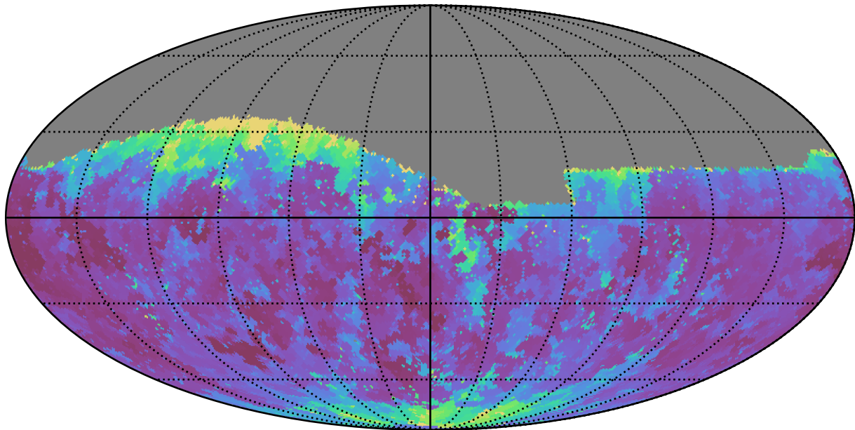
too_elab_r32_d2_gz_v3.4_10yrs Yr 1 g band: Min seeingGeom
