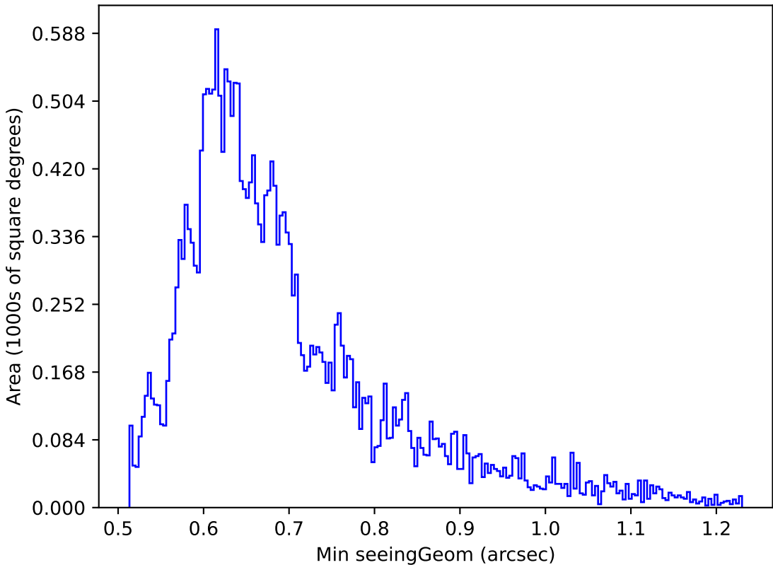
too_elab_r32_d2_gz_v3.4_10yrs Yr 1 g band: Min seeingGeom
