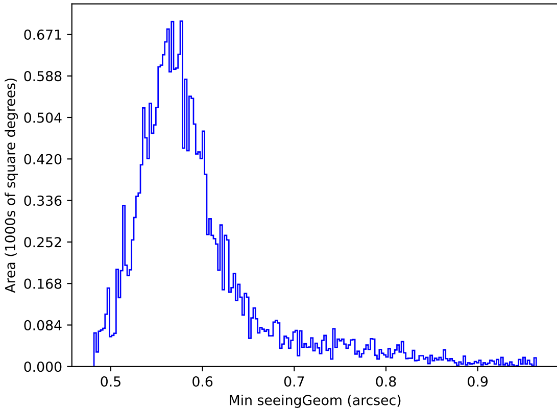
too_elab_r32_d2_gz_v3.4_10yrs Yr 1 all bands: Min seeingGeom
