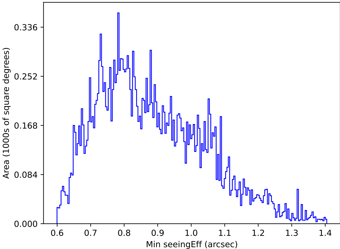
too_elab_r32_d2_gz_v3.4_10yrs Yr 1 u band: Min seeingEff
