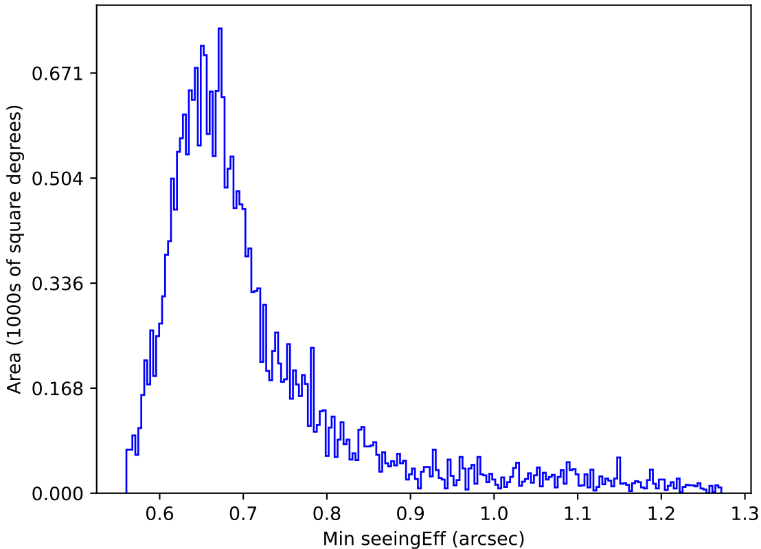
too_elab_r32_d2_gz_v3.4_10yrs Yr 1 i band: Min seeingEff
